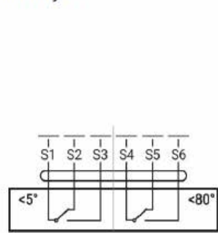
Auxiliary switch
