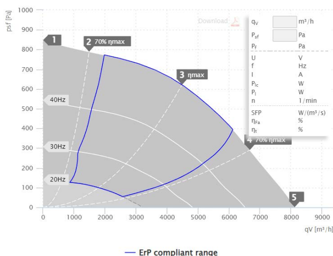
MPC 500 D4 T40 | 157233 (400V)
