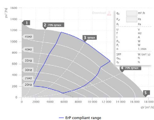
MPC 630 D4 T40 | 157241 (400V)
