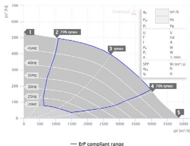
MPC 400 D4 T40 | 157231 (400V)
