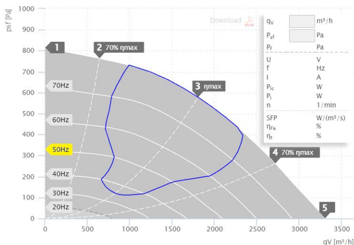
MPC 315 D4 T40 | 157224 (400V)
