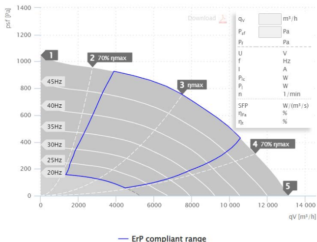
MPC 560 D4 T40 | 157235 (400V)
