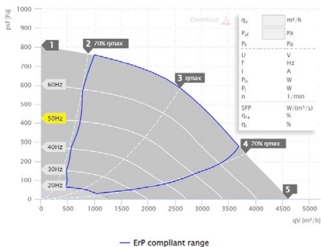
MPC 355 D4 T40 | 157226 (400V)
