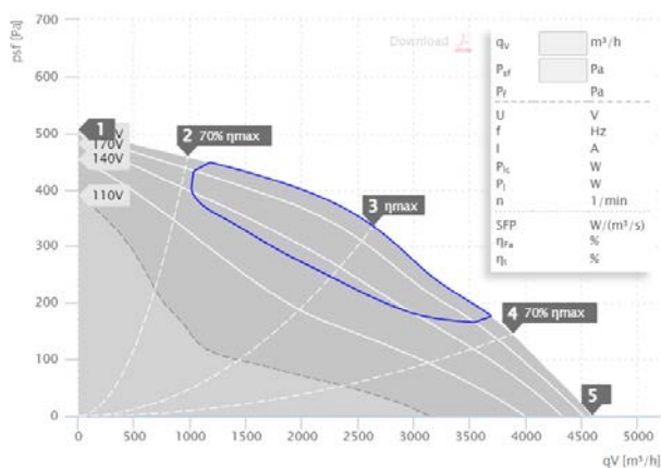
MPC 400 E4 T21 | 136887 (230V)
