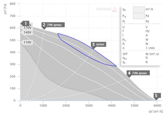
MPC 450 E4 T20 | 126624 (230V)
