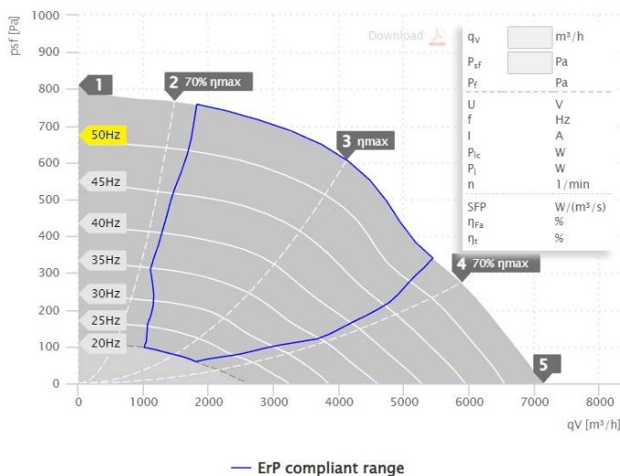
MPC 450 D4 T40 | 157232 (400V)
