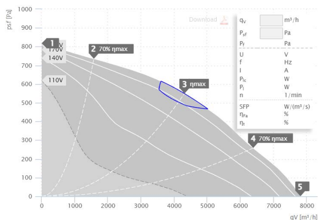
MPC 500 E4 T22 | 141186 (230V)
